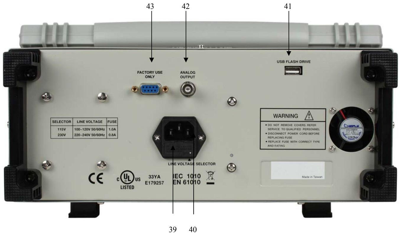
Fig. 2. Rear Panel Controls and Indicators.
