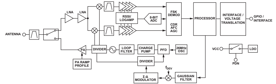
Figure 20: NT Series Transceiver Block Diagram
