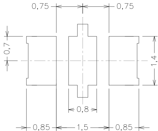
Soldering patterns
