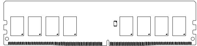
Figure 1: 288-Pin UDIMM (MO-309 R/C A1)
