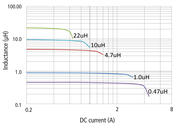
TYS252012L Typical L vs DC Current
