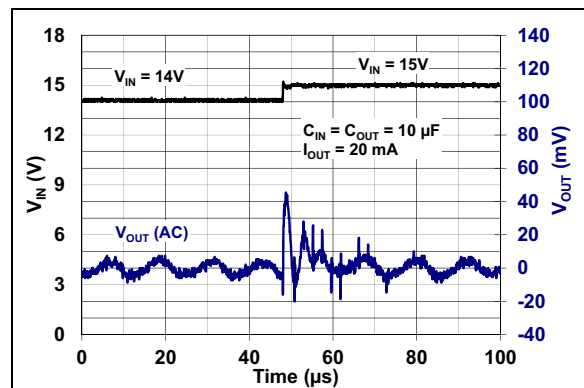
FIGURE 2-6: 5V LDO Dynamic Linestep – Rising V_{\text{DD}} .
