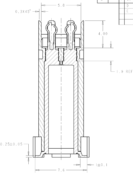
SECT A-A SCALE 8:1
