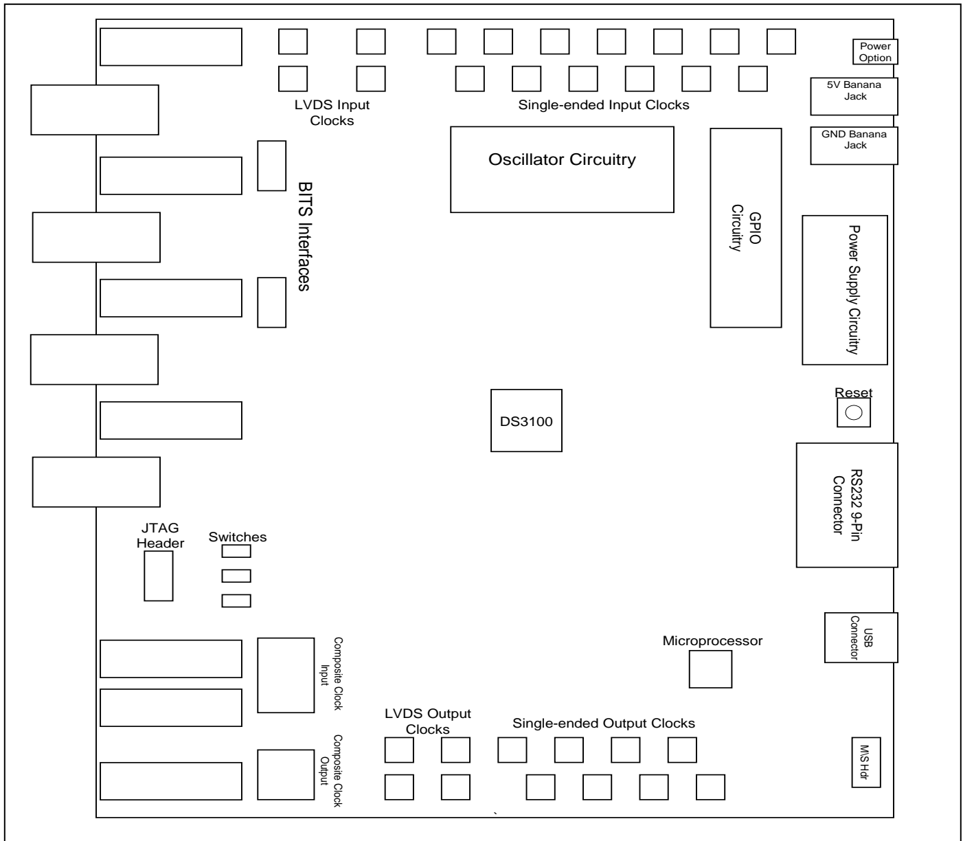
Figure 1-1. Board Floorplan
