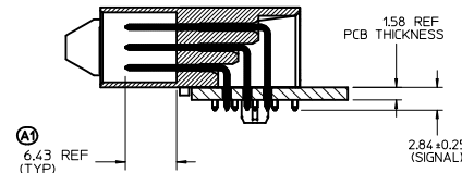
SECTION Z-Z
