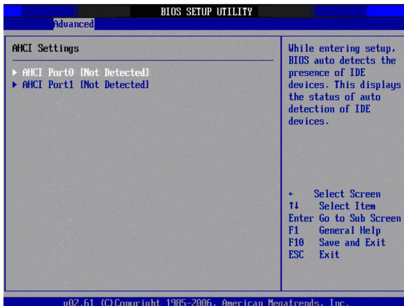
Figure 3.13 AHCI Configuration
