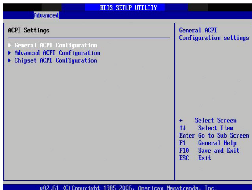
Figure 3.9 ACPI Settings
