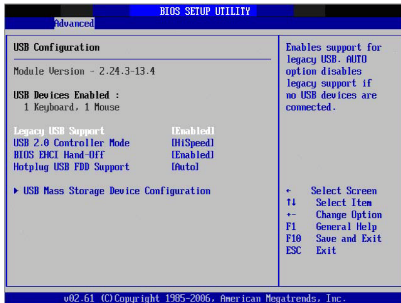
Figure 3.18 USB Configuration
