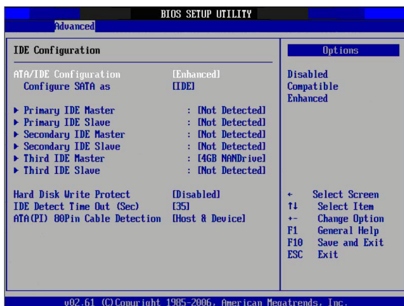
Figure 3.5 IDE Configuration
