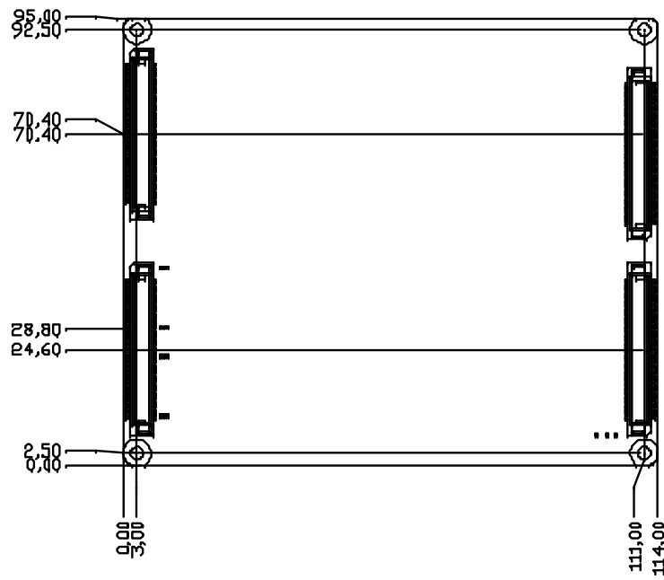
Figure 2.3 SOM-4463 B2 Rear Side
