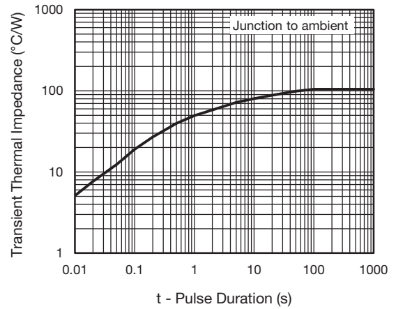
Fig. 7 - Thermal Resistance
