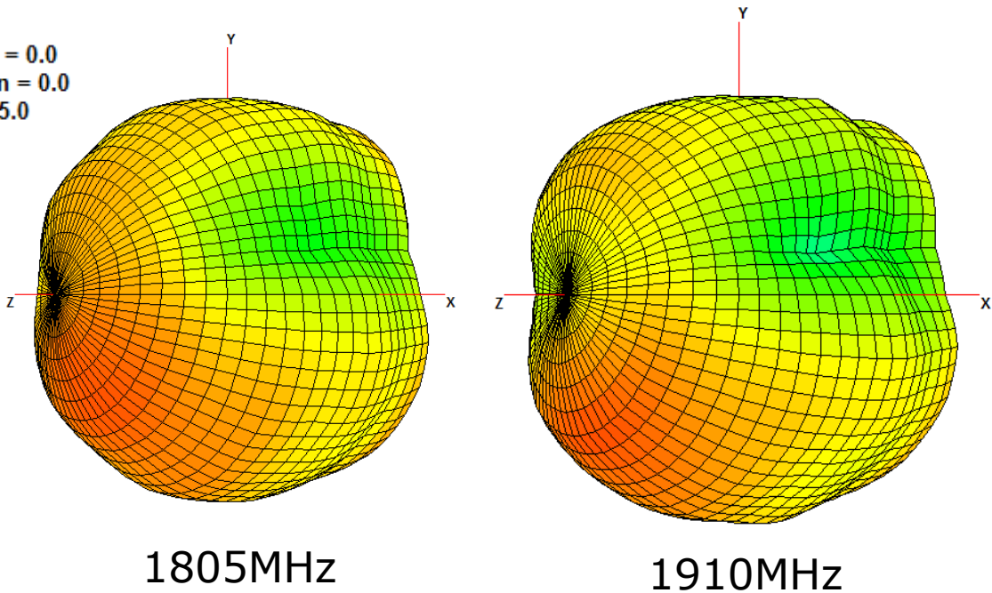
Figure 13. 3D Radiation Pattern at 1805 and 1910 MHz of the Warrior PA.711.A Antenna on MIMO PAD.71X.A
