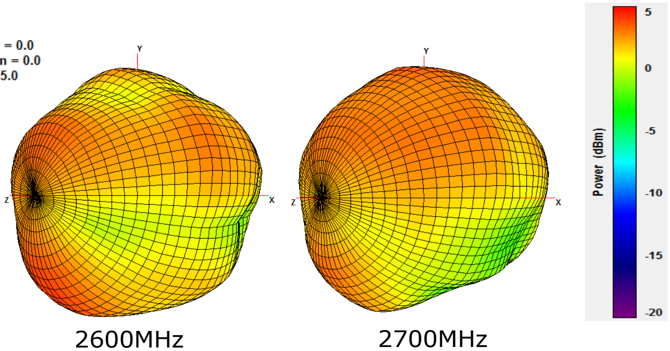
Figure 16. 3D Radiation Pattern at 2600 and 2700 MHz of the Warrior PA.711.A Antenna on MIMO PAD.71X.A
