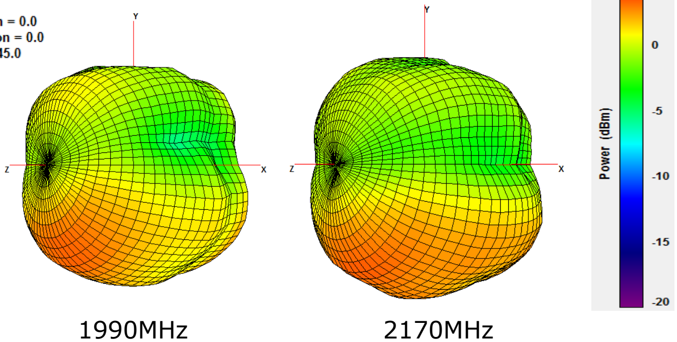
Figure 14. 3D Radiation Pattern at 1990 and 2170 MHz of the Warrior PA.711.A Antenna on MIMO PAD.71X.A
