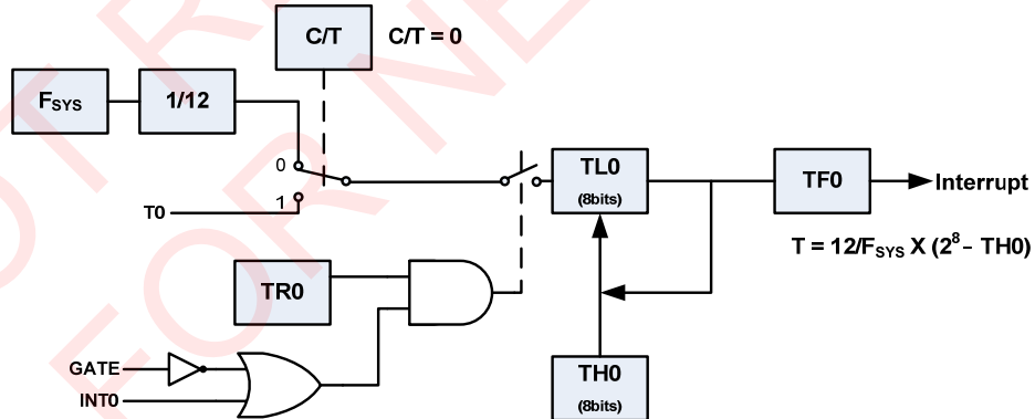
Figure 14 – Timer0 Mode2
