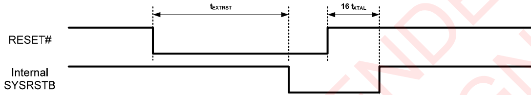
Figure 35 – RESET# Timing
