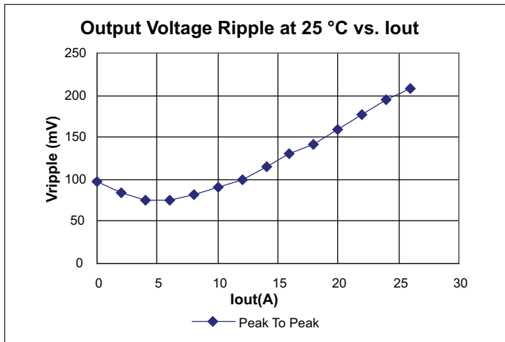
Figure 7 — Vripple vs. I OUT ; 352 V IN , no external capacitance
