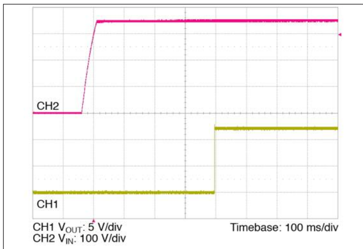
Figure 9 — V IN to V OUT start up waveform
