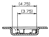
SECT E-E
