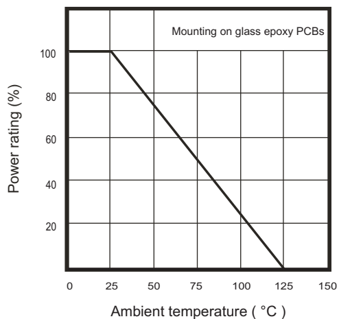
Fig. 3 - Power rating derating curve
