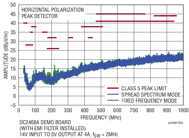
Figure 4. LT8645S Demo Circuit DC2468A EMI Performance (14V Input from VEMI, with EMI Filter, I_{OUT} = 4A )
