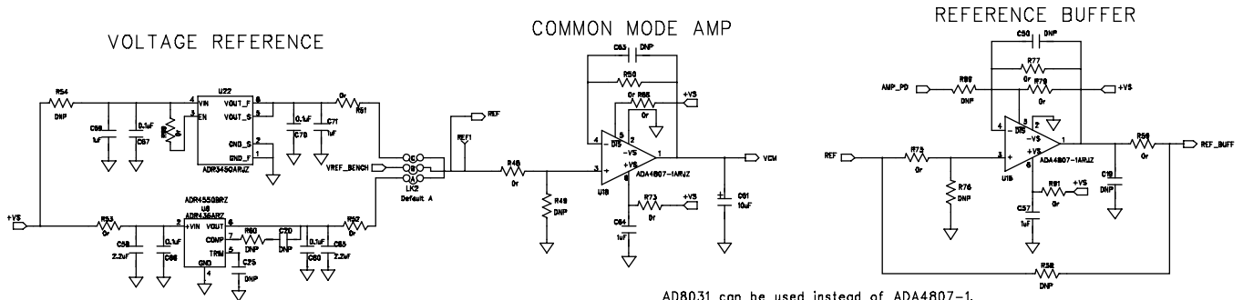
Figure 26. ADC Evaluation Board, Voltage Reference, Common-Mode and Reference Buffers
