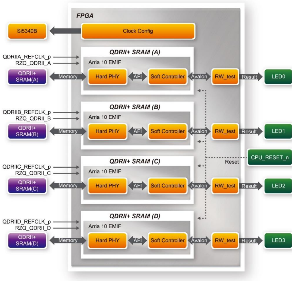
Figure 6-1 Function Block Diagram of the QDRII+ SRAM x4 Demonstration
