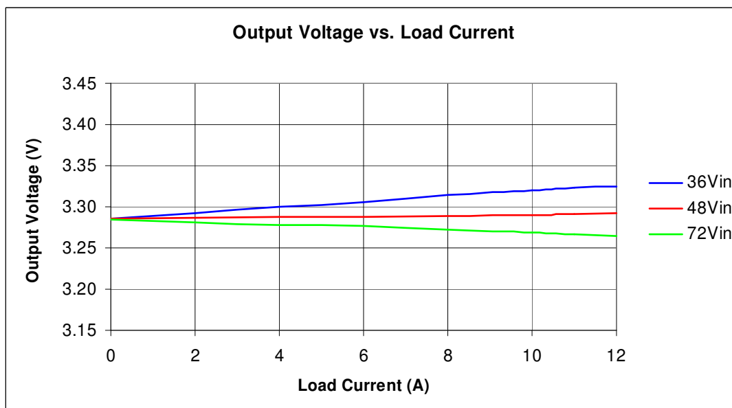
Figure 4. Regulation (400LFM)
