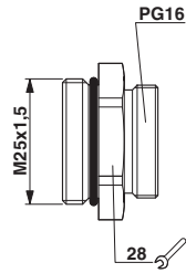
Dimensioned drawing
