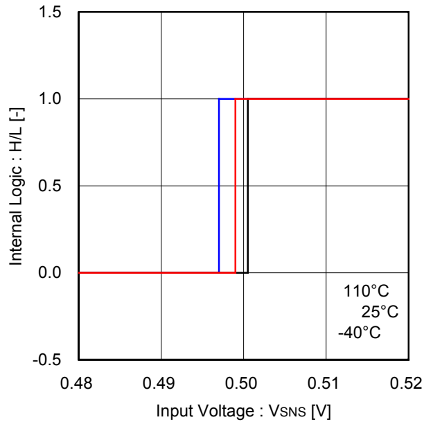
Figure 42. Current Limiter Input Threshold Voltage (SNS)
