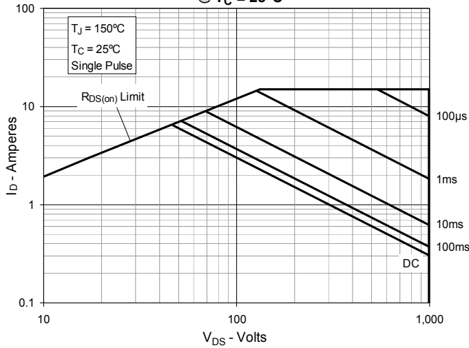
Fig. 15. Forward-Bias Safe Operating Area @ T_C = 25^\circ C
