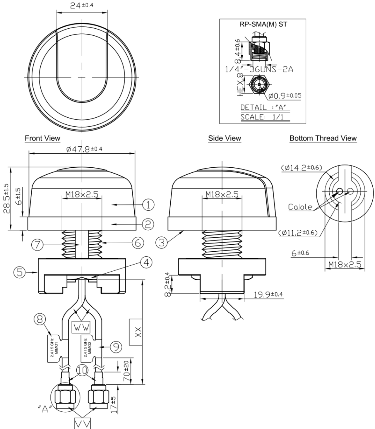
Figure 23. Antenna Drawing
