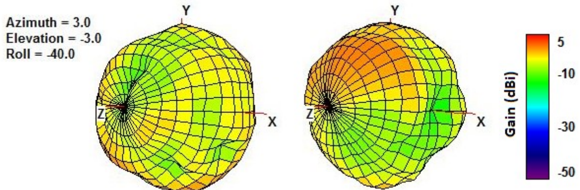
Figure 18. 3D Radiation Pattern at 2450 MHz (left side), Radiation Pattern at 5400 MHz (right side) of the MA550 Antenna
