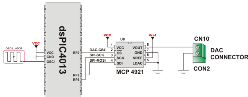
SPI HW connection
