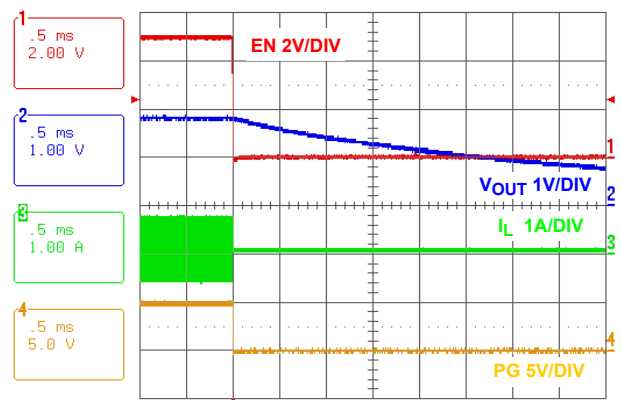
FIGURE 25. SOFT-DISCHARGE SHUTDOWN
