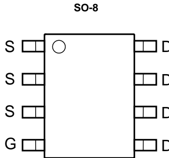
Top View Internal Schematic
