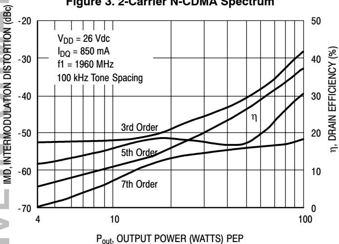
Figure 5. Intermodulation Distortion Products versus Output Power
