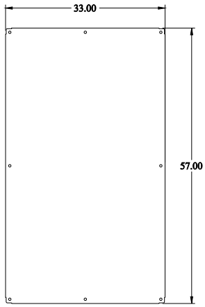
INNER PANEL
