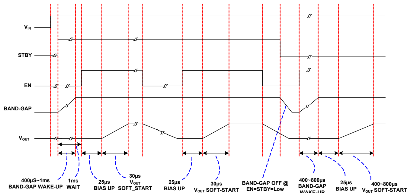
FIGURE 23. TIMING DIAGRAM
