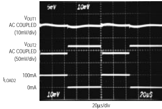
CROSTALK DUE TO LOAD TRANSIENT
