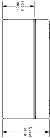
SIDE VIEW OF ENCLOSURE
