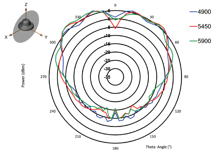
Vertical Plane - 4900-5900 MHz
