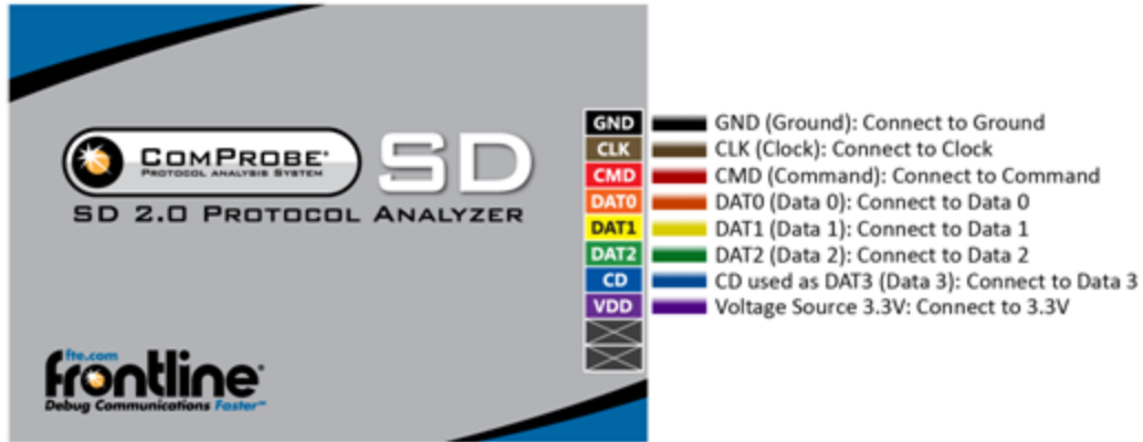
Figure 2.7 - Pin Header
