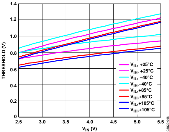
Figure 19. Typical \overset{P}{C} Thresholds ( V_{IH} and V_{IL} )
