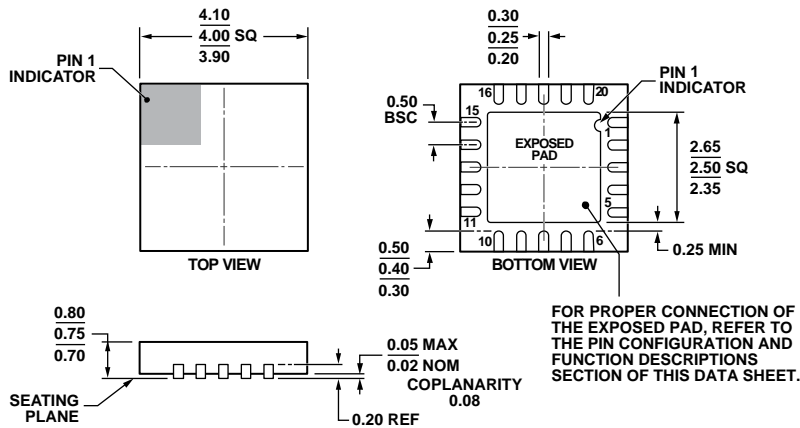
COMPLIANT TO JEDEC STANDARDS MO-220-WGGD. Figure 55. 20-Lead Lead Frame Chip Scale Package [LFCSP_WQ] 4 mm x 4 mm Body, Very Very Thin Quad (CP-20-10) Dimensions shown in millimeters
