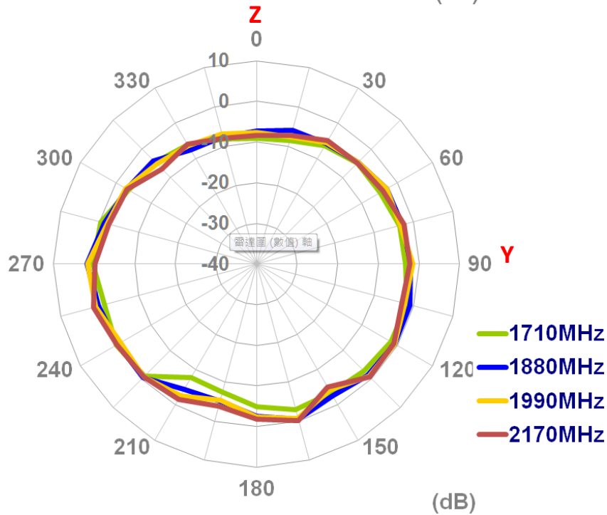
Figure 6. 2D Radiation Pattern of the TG.22 Antenna.
