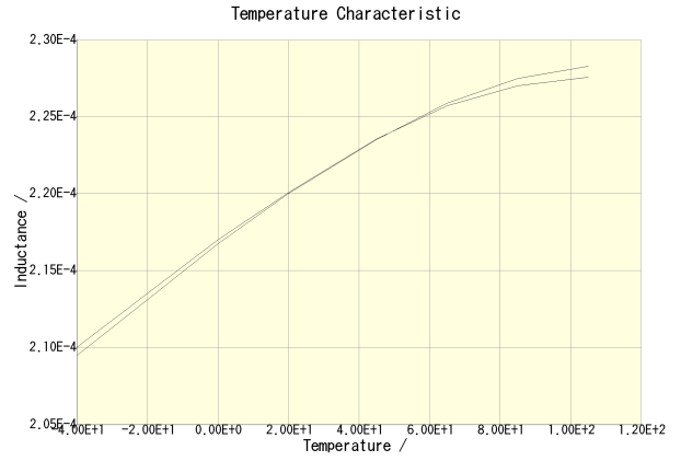
CLF12555T-221M-CA(DC = 0A)
