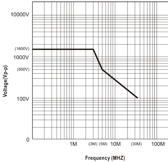
Figure 1. CT4076-NA Derating Curve
