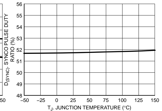
Figure 15. SYNCO Pulse Duty Ratio vs. Junction Temperature
