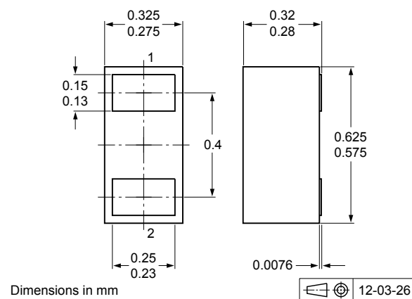
Fig. 22. Package outline DSN0603-2 (SOD962)
