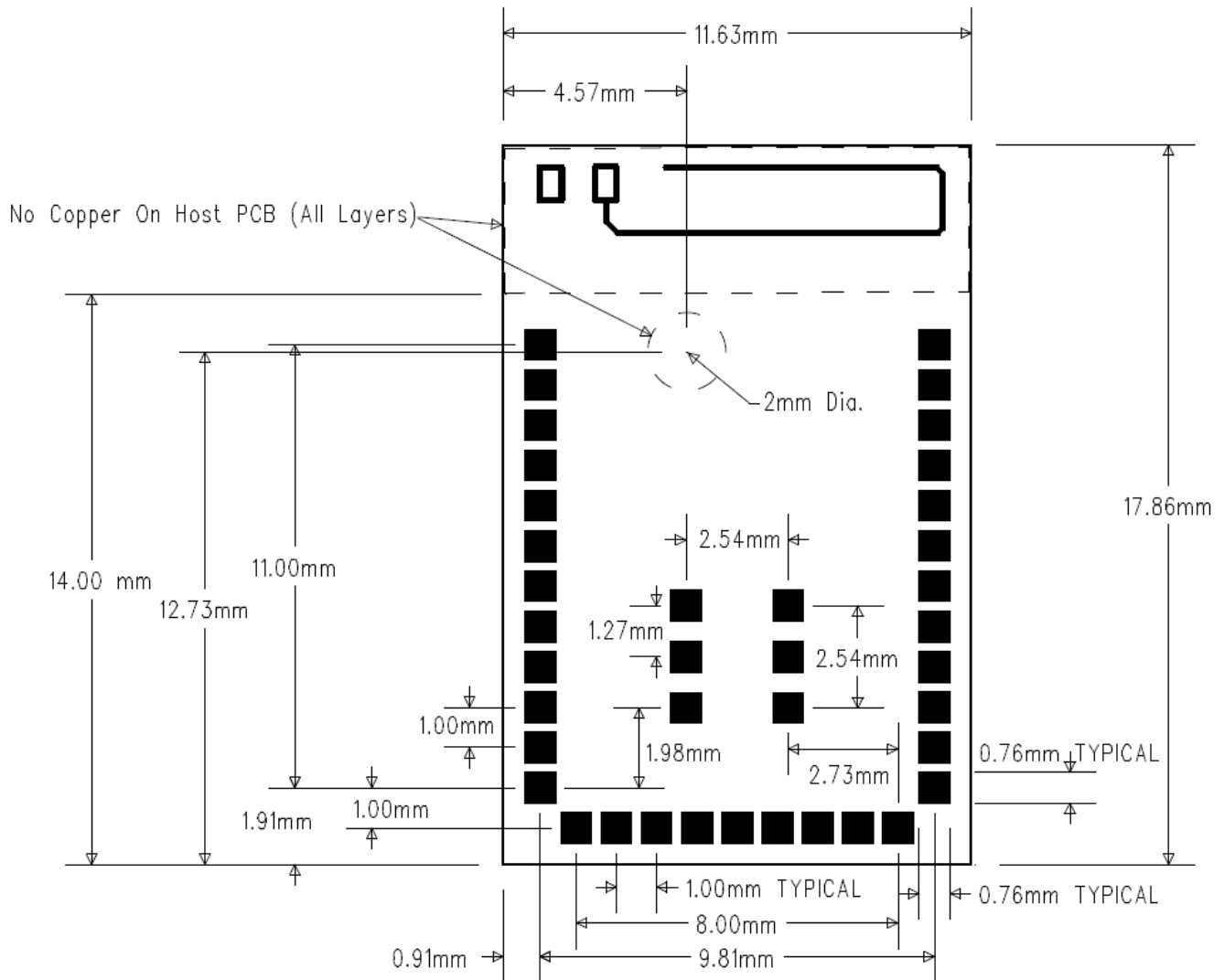
Figure 20 SaBLE-x Recommended PCB Footprint (Viewed from Top)
