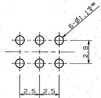
Reference dimension drawing of mounting hole 取付穴推奨寸法図 (Tolerance 公差: ±0.05) (t=0.8mm)
