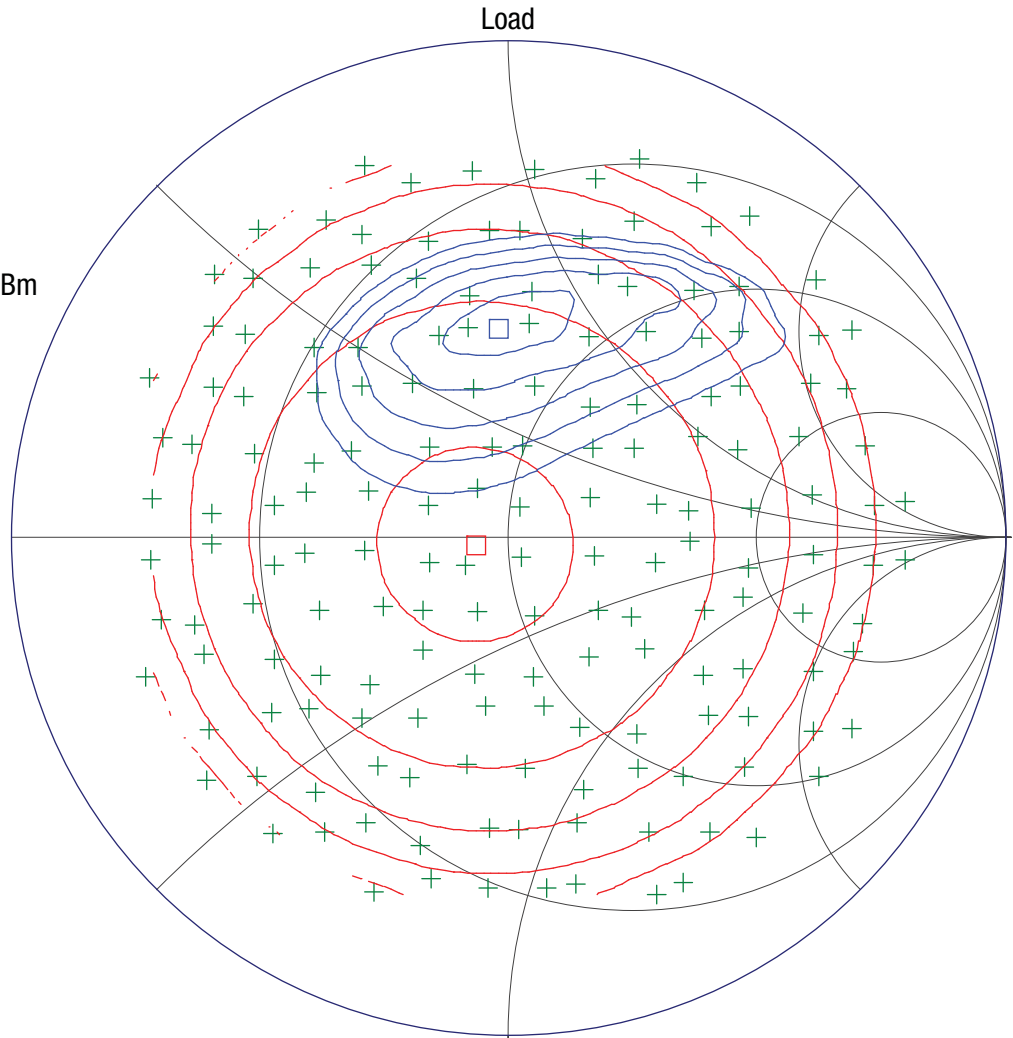
Figure 20. OIP3 Load Pull @ 800 MHz, 5 V, 70 mA (Input Load = Min NF, -20 dBm/tone, 5 MHz Spacing)
