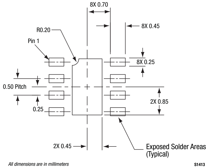
Figure 26. SKY67153-396LF PCB Layout Footprint (Top View)
