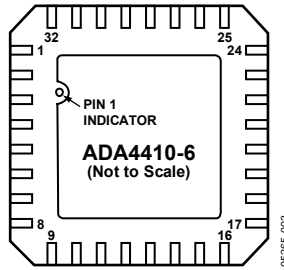
Figure 3. 32-Lead LFCSP Pin Configuration, Top View
