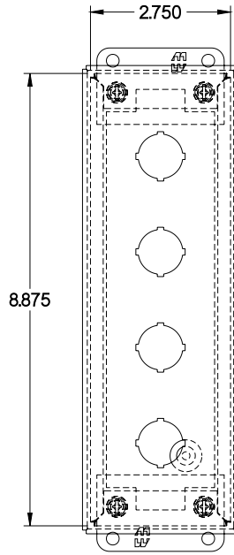
FRONT VIEW
