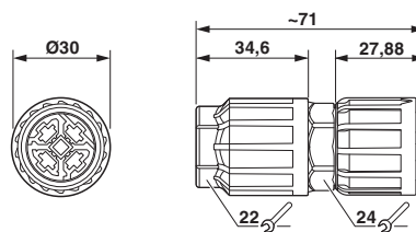
Dimensional drawing
