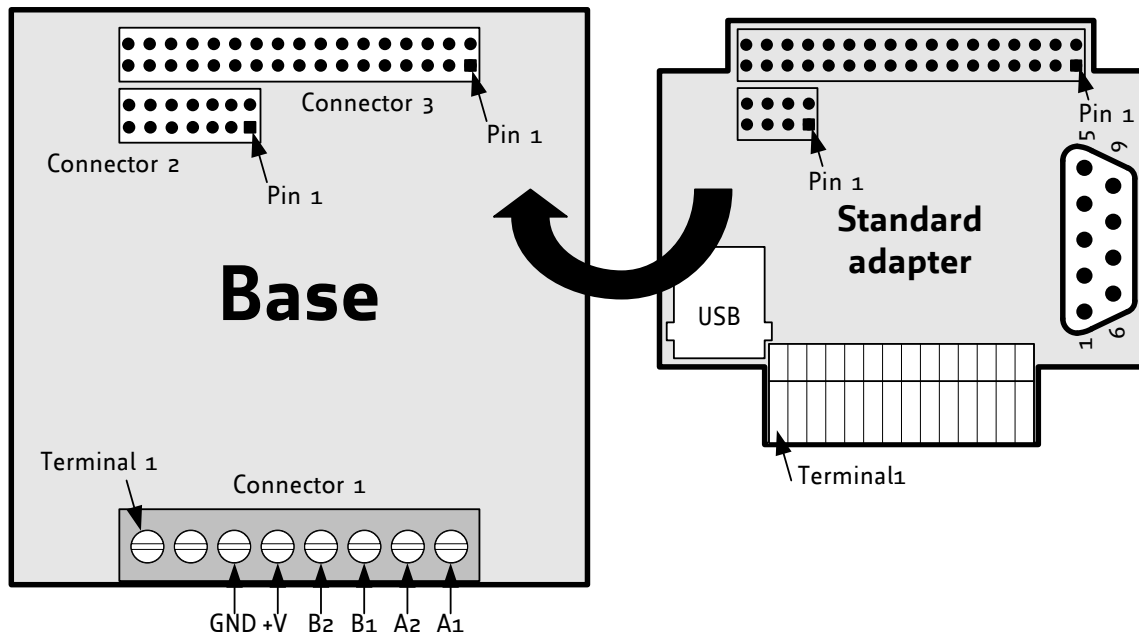
Figure 4.2: Connectors of the TCM-142
