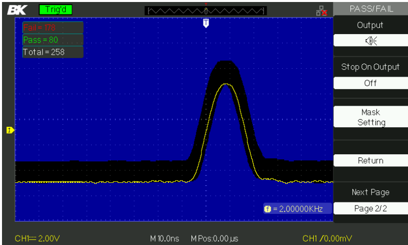
Figure 3.64 – Pass/Fail Screen 2
