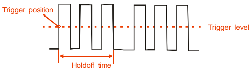
Figure 3.29 – Trigger Holdoff Illustration
