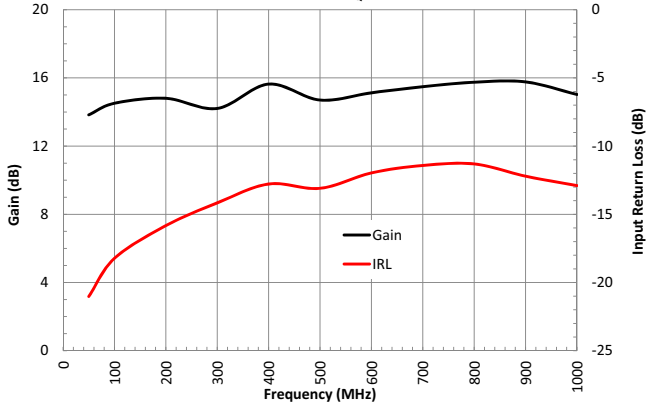
Gain/IRL versus Frequency, P OUT = 41dBm (CW, V_D = 28V, I_{DQ} = 88mA )
