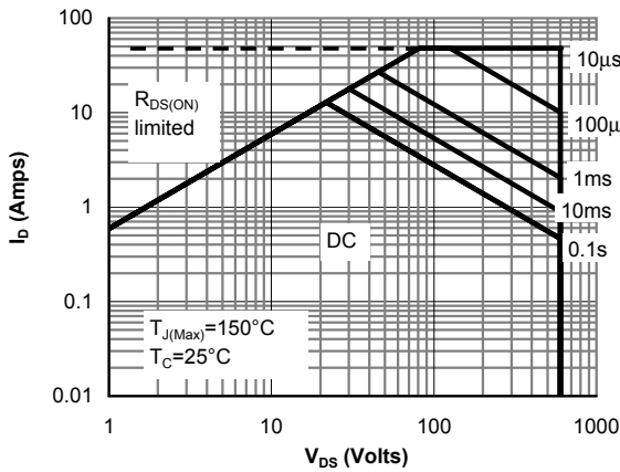
Figure 9: Maximum Forward Biased Safe Operating Area for AOT12N60FD (Note F)
